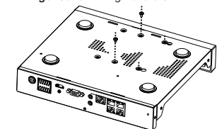
Figure3-3 Fixing hard disk
