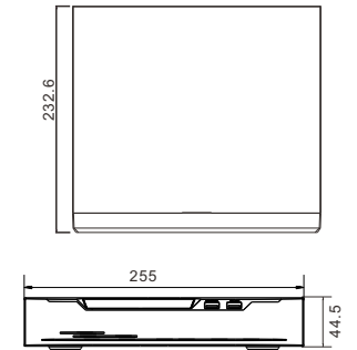
Figure 2-1 Dimensions (Unit:mm)
